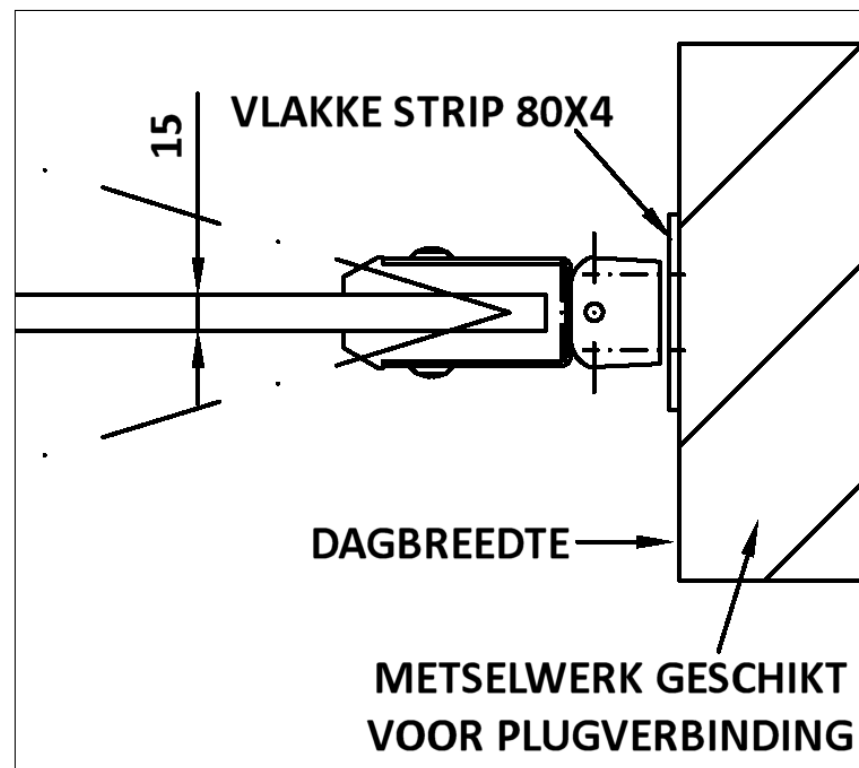
DETAIL X
