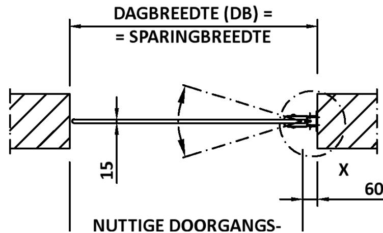
DETAIL X
